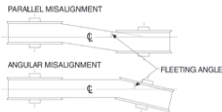
Figure 3 - Misalignment between belt and sheave is a major cause of abnormal V-belt wear.
