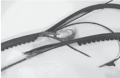
Figure 1 - Normal V-belt failure is characterized by a break or separation.
