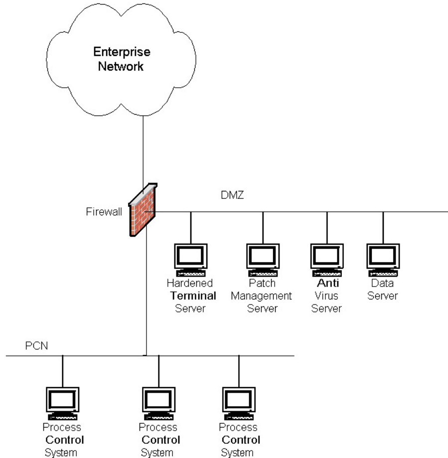
Figure A – Generic and Simplified Representation of an Interface between a PCN and an Enterprise Network
